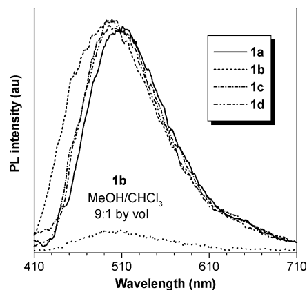
Figure 8. Photoluminescence spectra of hyperbranched poly(phenylenesilole)s 1a–1d in THF and 1b in a methanol/chloroform mixture (9:1 by volume) at room temperature; [ 1 ] = 10 \mu\text{g/mL} , \lambda_{\text{ex}} = 407 nm.
