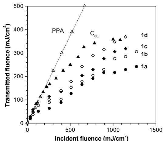
Figure 7. Optical responses to 8 ns, 10 Hz pulses of 532 nm laser light, of dichloromethane solutions (0.70 mg/mL) of hyperbranched poly(phenylenesilole)s. Data for poly(phenylacetylene) (PPA) and \text{C}_{60} solutions are shown for comparison. Linear transmittance (%): 70 ( 1a ), 80 ( 1b ), 82 ( 1c ), 85 ( 1d ), 79 ( \text{C}_{60} ), 75 (PPA).
