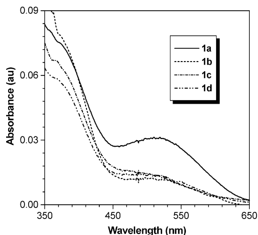
Figure 5. UV spectra of THF solutions (10 \mu\text{g/mL} ) of hyperbranched poly(phenylenesilole)s.
