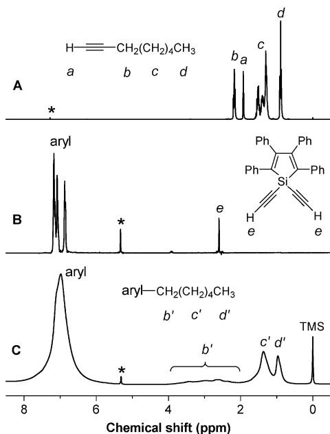
Figure 3. ^1\text{H} NMR spectra of (A) 1-octyne 3 (in \text{CDCl}_3 ), (B) silolyldiyne 2 (in \text{CD}_2\text{Cl}_2 ), and (C) their polymer 1b (in \text{CD}_2\text{Cl}_2 ). The solvent peaks are marked with *.
