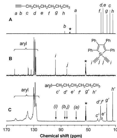
Figure 4. ^{13}\text{C} NMR spectra of (A) 1-octyne 3 (in \text{CDCl}_3 ), (B) silolyldiyne 2 (in \text{CD}_2\text{Cl}_2 ), and (C) their polymer 1b (in \text{CD}_2\text{Cl}_2 ). The solvent peaks are marked with *.
