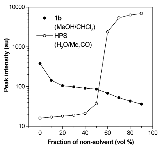
Figure 9. Peak intensity of photoluminescence of 1b vs solvent composition of methanol/chloroform mixture at room temperature; [ 1b ] = 10 \mu\text{M} , \lambda_{\text{ex}} = 407 nm. Data for 1,2,3,4,5,6-hexaphenylsilole (HPS) in water/acetone mixtures are shown for comparison.
