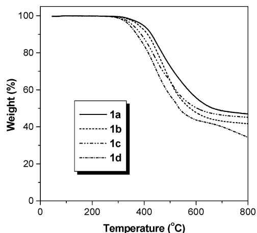
Figure 6. TGA thermograms of hyperbranched poly(phenylenesilole)s.
