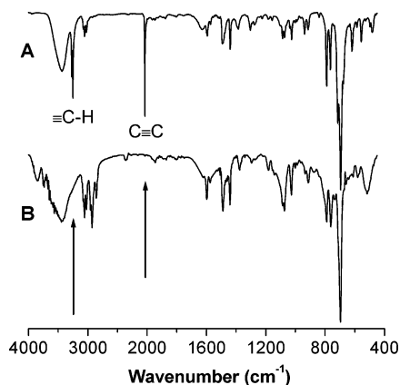
Figure 2. IR spectra of (A) silolyldiyne 2 and (B) its polymer 1b .
